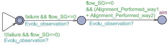
Fig. 6. Observer for process specification ( S_{PE} )
