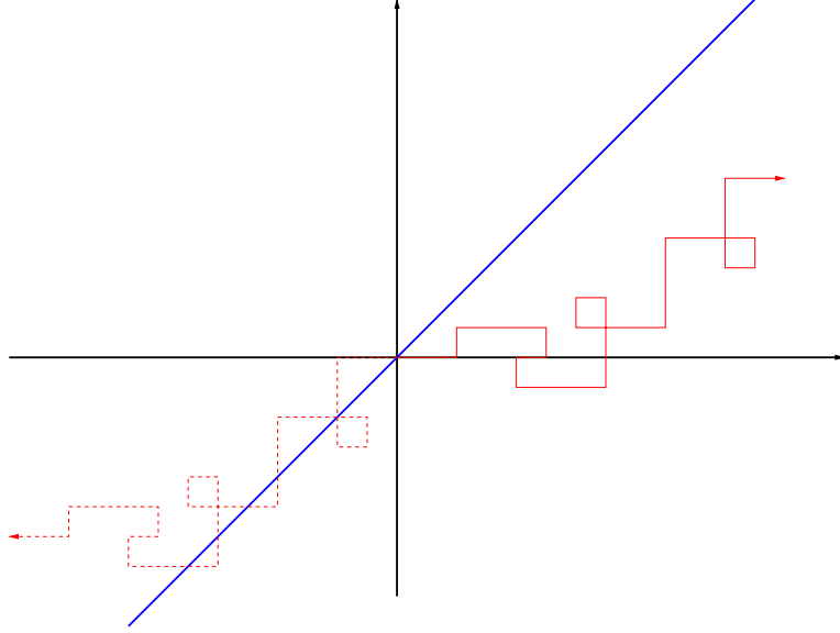
The paths \eta (in red) and \beta(\eta) (in dashed red)
