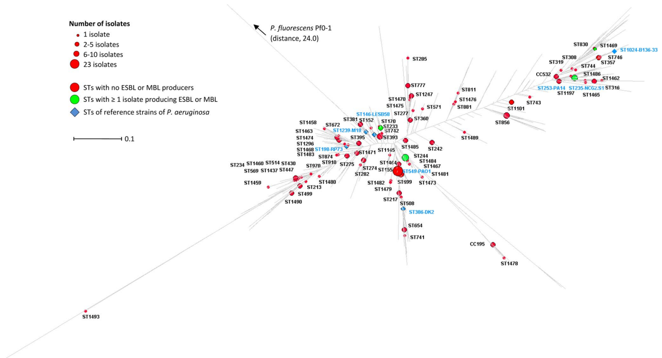
Figure 2. Distribution of the STs and CCs of the 184 clinical isolates of Pseudomonas aeruginosa isolated in West and Central Africa on a dendrogram built with the data all known STs ( n=1595 ). STs without any isolates producing ESBL or MBL were represented with red spots. STs represented by \geq 1 isolate producing ESBL or MBL were represented with green spots. STs of reference isolates are represented with blue diamonds. The dendrogram is based on the alignment of the concatenated sequences of the acsA , aroE , guaA , mutL , nuoD , ppsA and trpE genes (forming an artificial 2,882-bp sequence) of the 1595 STs of the P. aeruginosa MLST database in July 2013 [11]. See Material and methods section for details.
