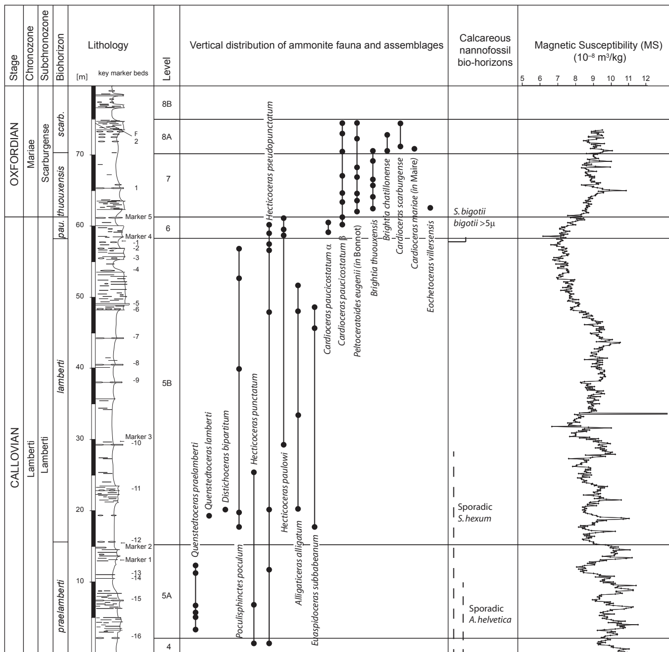
Fig. 4. Detailed lithology, biostratigraphy and distribution of ammonite fauna, calcareous nannofossils and magnetic susceptibility, for the Saint-Pierre d'Argeçon section
