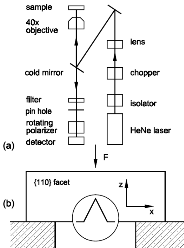
Fig. 1: Schematic diagram of the measurement apparatus and of the calibration bar.
