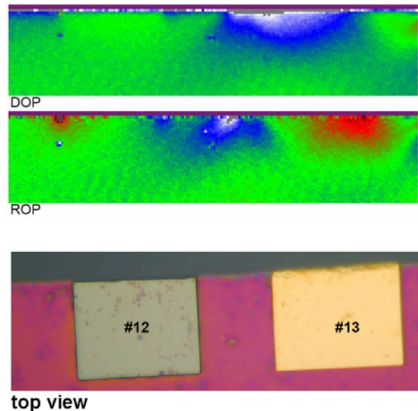
Fig. 6: Maps of the DOP and ROP over an area of 180 \mu\text{m} \times 40 \mu\text{m} on the facet for a cleave through a pcm area. An image of the top of the pcm area is shown.
