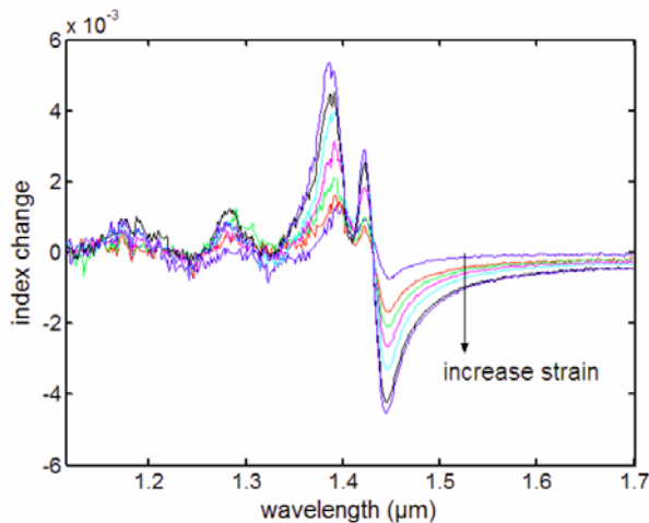
Fig. 4: Refractive index as a function of wavelength and for increasing strain.
