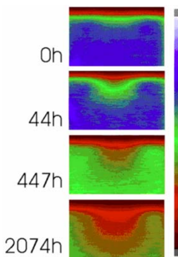
Fig. 3: Maps of the PL yield as a function of time on accelerated aging. The active region is at the top.
