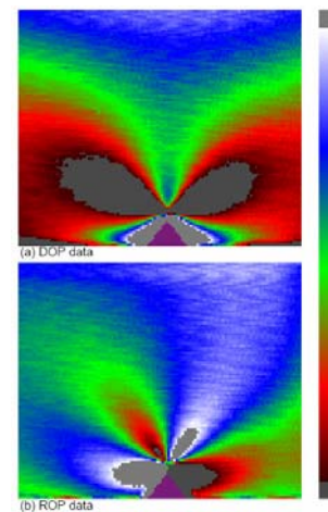
Fig. 2: Maps of the DOP and ROP near a v-groove of the calibration bar of Fig. 1(b) for a non-zero F .
