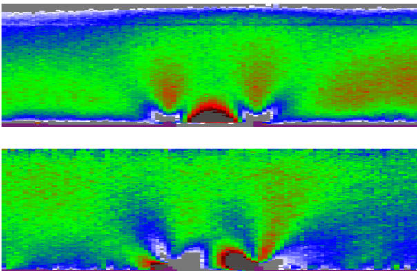
Fig. 7: Measured DOP (top) and ROP (bottom) from the facet of a bonded cm-bar laser.
