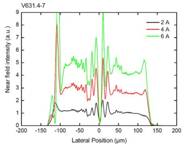
Fig. 5: Predicted near field of a broad area laser. The simulation included index variations that were estimated from DOP measurements.
