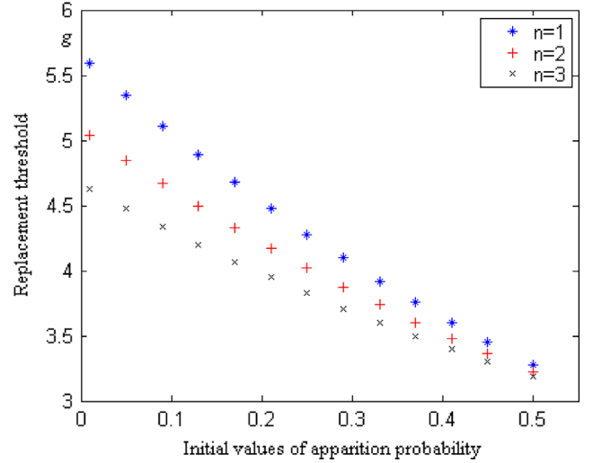
Fig. 2. Impact of the new technology appearance probability on the replacement threshold for the three first decision periods.
