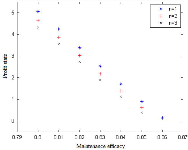
Fig. 4. The effect of maintenance efficacy on the replacement threshold in non-obsolescence case.
