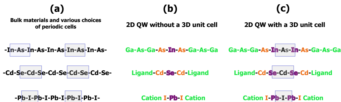
Figure 6. Schematic view of the periodic bonding along the nearest-neighbor axis for a) InAs and CdSe zinc-blende bulk crystals, and (CH 3 NH 3 )PbI 3 bulk, b) ultrathin layers, c) thin QW with interface layers.
