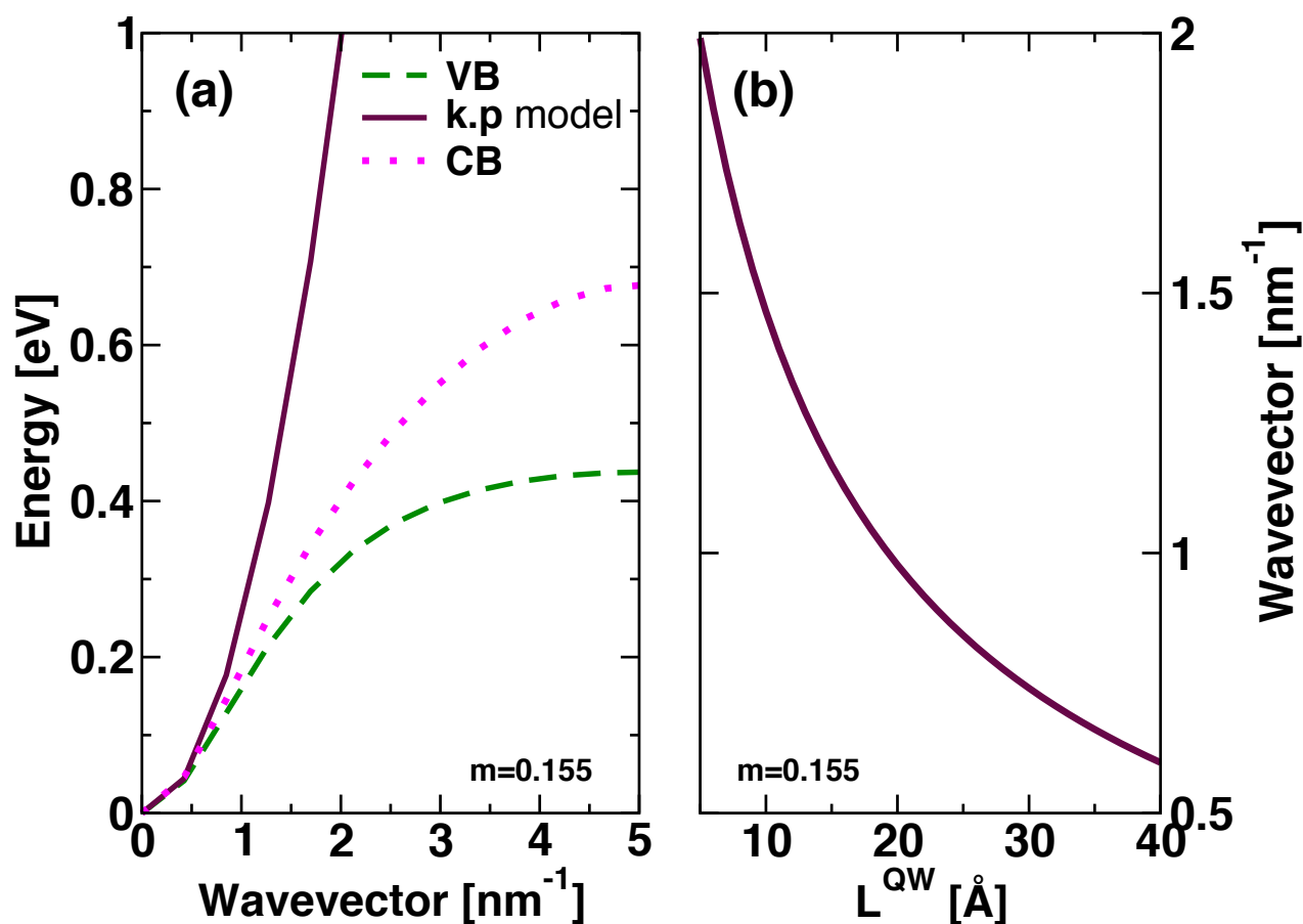
Figure 7. a) Energy dispersion of the VB (dashed line) and CB (dotted line) ground states for the low temperature phase of the 3D bulk reference material (CH 3 NH 3 )PbI 3 . The straight line is the parabolic dispersion obtained when considering an effective mass of 0.155. b) QW wavevector computed for various QW thicknesses using the same effective mass.
