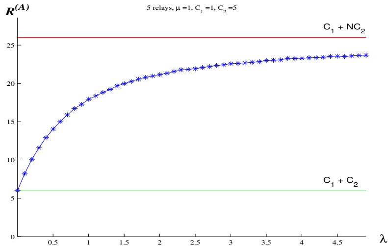
Figure 1: Expected reward paid by the source for the adaptive strategy. N = 5 , \mu = 1 , C_1 = 1 , C_2 = 5 .
