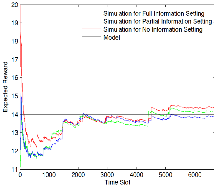
Figure 7: Expected reward under three static strategies: full information, partial information and no information for N = 10 , \mu = 0.1001 , \lambda = 0.2541 , C_1 = 3 , C_2 = 1.0999 .
