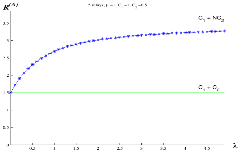
Figure 2: Expected reward paid by the source for the adaptive strategy. N = 5 , \mu = 1 , C_1 = 1 , C_2 = 0.5 .
