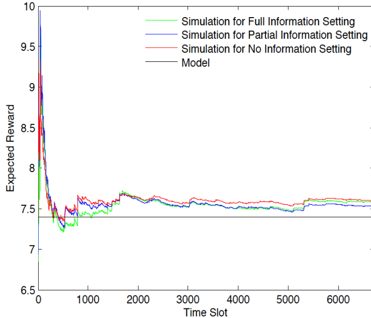
Figure 6: Expected reward under three static strategies: full information, partial information and no information for N = 4 , \mu = 0.1 , \lambda = 0.2547 , C_1 = 3 , C_2 = 1.1 .
