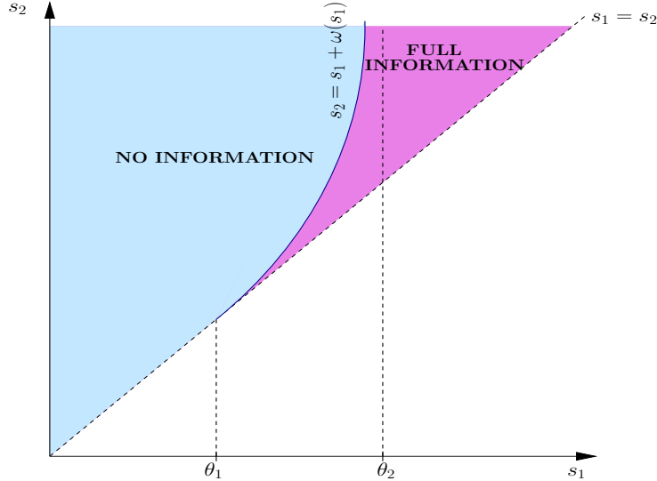
Figure 3: Optimal strategy for the source for \lambda > \mu .
