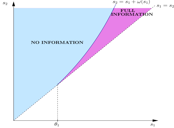
Figure 4: Optimal strategy for the source for \lambda < \mu .
