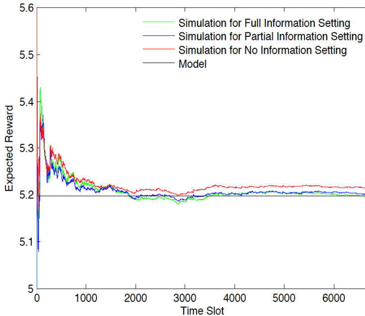
Figure 5: Expected reward under three static strategies: full information, partial information and no information for N = 2 , \mu = 0.0998 , \lambda = 0.2542 , C_1 = 3 , C_2 = 1.1002 .
