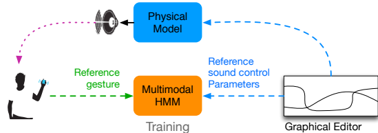
(a) Training : sounds are designed using a graphical editor, and reference gestures can be recorded while listening.
