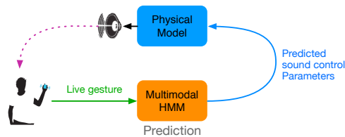
(b) Performance : the model is used to predict the sound parameters associated with a live gesture.
