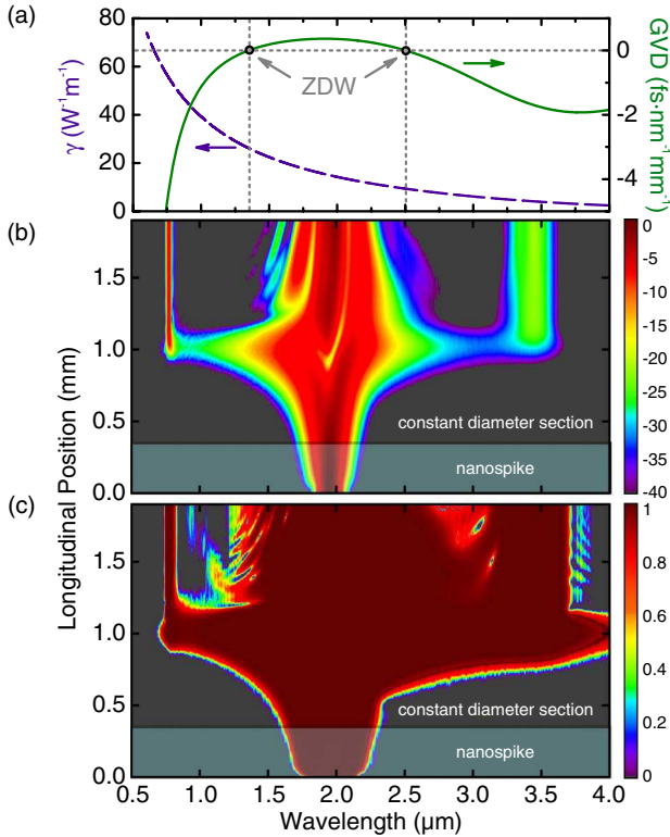
Fig. 4. Simulation of optical properties and supercontinuum generation inside the chalcogenide-silica waveguide. (a) Spectral dependence of nonlinear coefficient (dashed purple curve) and group velocity dispersion (solid green curve) within the constant diameter section. The two zero-dispersion wavelengths (ZDWs) are highlighted by the two grey dotted vertical lines. (b) Generated supercontinuum spectrum at different longitudinal positions within the fiber (color scale is the normalized spectrum in decibels). (c) Corresponding degree of first-order coherence (color scale is linear, 1 is full coherence with the pump laser). The region of propagation within the nanospike is indicated by the light grey sections in (b) and (c).
