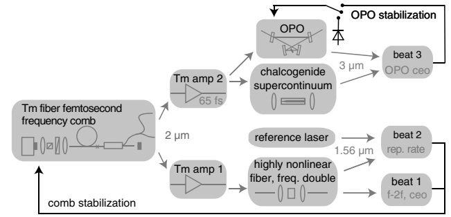
Fig. 6. Schematic of optical and electrical signals for phase locking of the doubly resonant OPO. All the resulting frequency combs in the near and mid-IR are coherently locked to the optical reference.
