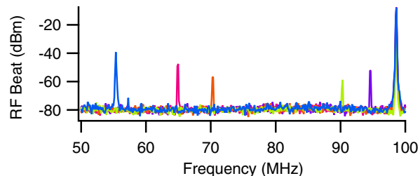
Fig. 3. Measured interference in the radio frequency spectrum of overlapped supercontinuum and dither-locked OPO pulses. The repetition rate is at 98.6 MHz; other peaks are beat frequencies. Different colors correspond to different OPO cavity lengths, which have different wavelengths. The presence of strong beats shows that the supercontinuum is coherent.
