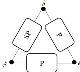
Fig. 1. Passivity maps of the system
