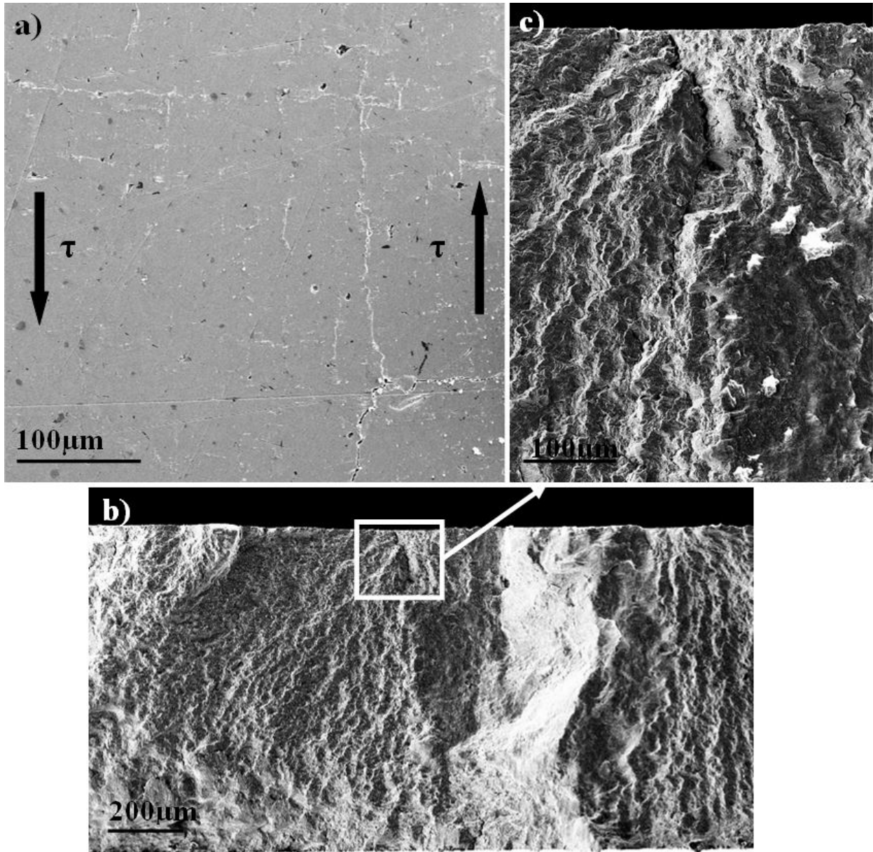
Fig. 10: a) Observation on the surface of a shear specimen showing crack initiation in the material matrix on planes at 0° and 90° to the specimen axis, b-c) failure surface for a shear test
