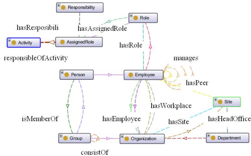
Figure 4: Part of the domain ontology defining the organization
