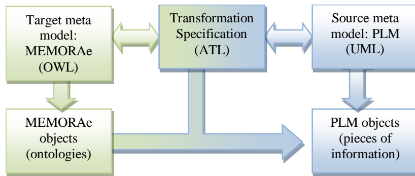
Figure 5: The aimed semantic interoperability
