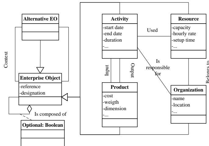
Figure 2: Product-Activity-Resource-Organization meta-model (Le Duigou et al., 2012)
