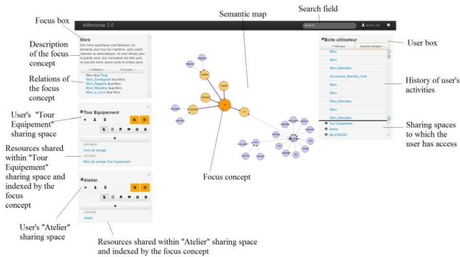
Figure 3: The main communication interface of the MEMORAe project web platform
