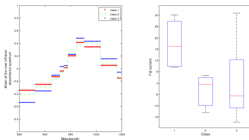
FIGURE 15. Summarized results for the model 2. The graph on the left is a candidate for representing each cluster, constructed by the mean of reconstructed spectrum over an a posteriori probability greater than 0.6. On the right side, we present the boxplot of the fat values in each class, for observations with an a posteriori probability greater than 0.6.
