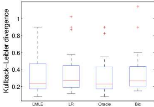
FIGURE 5. Boxplots of the Kullback divergence between the true model and the one selected by the procedure over the 20 simulations, for the Lasso-MLE procedure (LMLE), the Lasso-rank procedure (LR), the oracle (Oracle), the BIC estimator (BIC) for the model 2.
