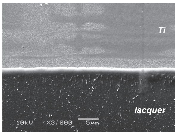
Fig. 9. Dynamic etching of lacquer on a Ti film, 4 to 6 shots, \lambda=248 nm, F=490 \text{ mJ.cm}^{-2} . Note the presence of some residues of the lacquer after autocombustion at the top left and the Ti film surface at the top right (SEM picture).
