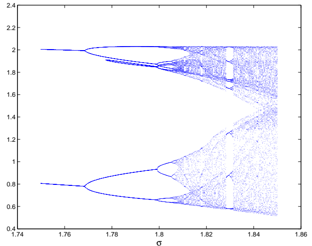
Fig. 1. Bifurcation diagram
