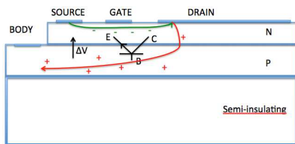
Figure 5: carrier mobility behavior during high voltage in MESFET SiC
