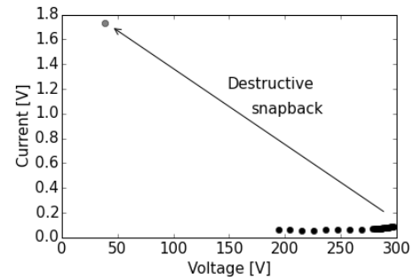
Figure 2: Id-Vd curve; Snapback occurs at a voltage above 300V during TLP Test.
