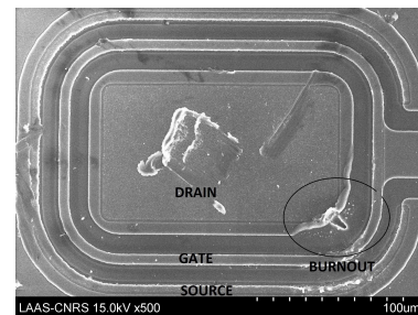
Figure 3: Damage observed at the corner of the SiC MESFET after TLP Stress (SEM photography).
