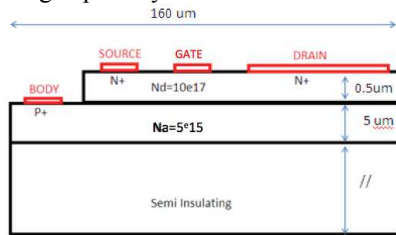
Figure 1: Schematic cross section of the studied SiC MESFET.
