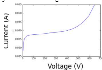
Figure 4: Id-Vd curve, above 600 Volts breakdown voltage observed with the 2D model of the MESFET simulating drain-source TLP Id(Vd) characteristic with floating gate and substrate.
