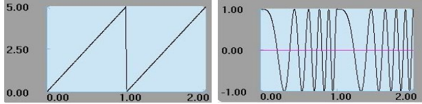
Fig. 5. FMCW SawTooth: Modulation (left), Signal (right)
