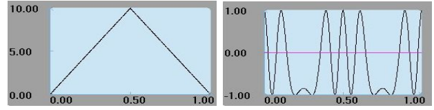
Fig. 7. FMCW Triangular: Modulation (left), Signal (right)
