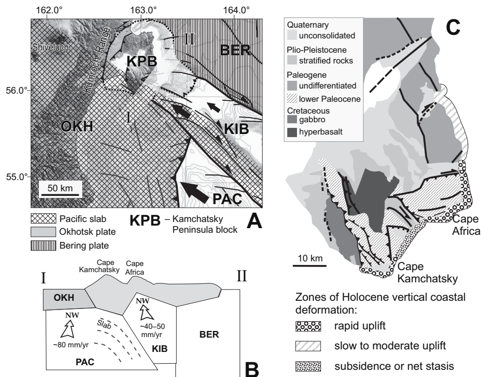
Figure 7. Proposed geodynamic model for the Kamchatsky Peninsula region. (A) Proposed boundary of Kamchatsky Peninsula block (KPB): Western onshore boundary is after Kozhurin (2009) and Kozhurin and Pinegina (2011); other boundaries are shown schematically; southern boundary is after Bourgeois et al. (2006) and Pedoja et al. (2006); northern and eastern boundaries are shown along the base of the continental slope (margin). I-II—position of the schematic cross section shown on B. (B) Schematic cross section of the Kamchatsky Peninsula region divided into plates. PAC—Pacific plate, BER—Bering plate, OKH—Okhotsk plate, KIB—Komandorsky [Commander] Island block. Okhotsk and Pacific plates extend to the northwest, Komandorsky Island and Bering plates are limited by the Kamchatsky Peninsula block. (C) Geological map of Kamchatsky Peninsula (modified from Freitag et al., 2001), showing its main structural features and main faults, both active and old and zones of Holocene vertical coastal deformation. Note that the faults in C are based on different interpretations than in A.
