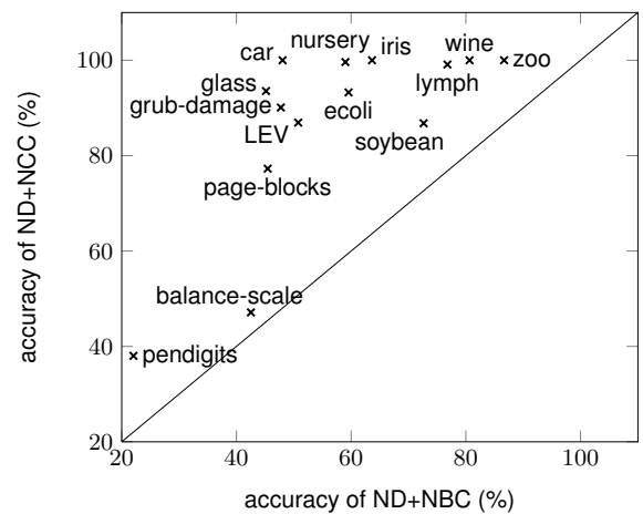
Figure 4. Accuracy of the methods “ND+NBC” and “ND+NCC” when a imprecise prediction is made by “ND+NCC”.
