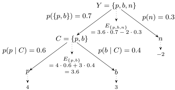
Figure 2. Expectation computation for c_n - c_p .
