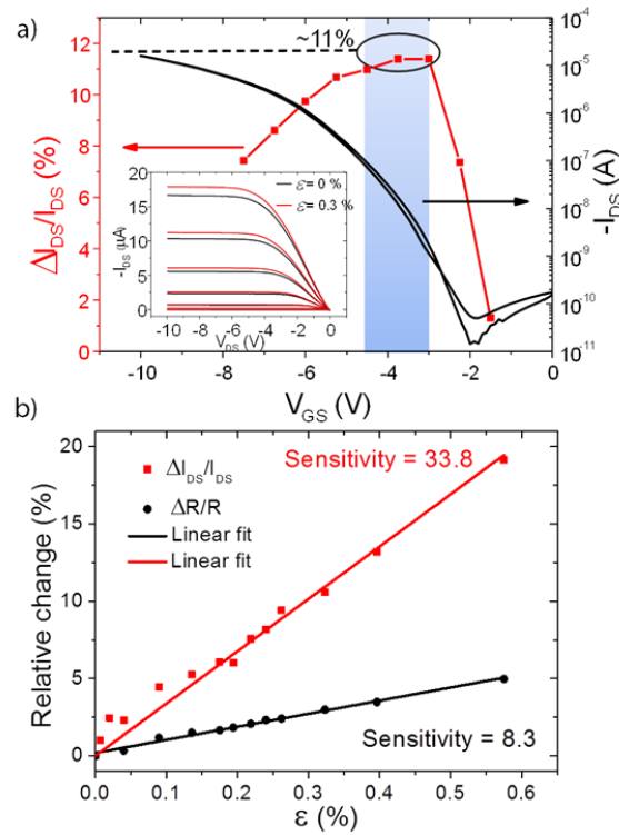
FIG. 2. a) Transfer characteristic of the OFET (black curve) and relative change of I_{DS} as a function of V_{GS} for a strain of \epsilon = 0.3\% (red curve); inset: output characteristic of the OFET between initial position and under 0.3% of applied strain at different V_{GS} ranging from -1.5V to -10V by steps of -0.75V, b) Amplification of the sensitivity of the piezoresistive MEMS using an OFET
