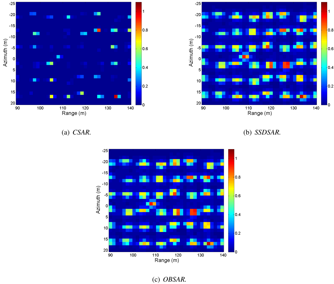
Fig. 13. SAR images for HH polarization using simulated FoPen data with a MMT located at position (108, -1)m. (a) The detection of the MMT in the CSAR image is not possible ( \rho_{CSAR} = -3.7\text{dB} ) and the false alarms due to the tree trunks are numerous. (b) Compared to CSAR, the MMT response in the SSDSAR image is increased but false alarms due to tree trunks are numerous and have high intensities ( \rho_{SSDSAR} = -0.5\text{dB} ). (c) The OBSAR gives the same image as the SSDSAR ( \rho_{OBSAR} = -0.5\text{dB} ).
