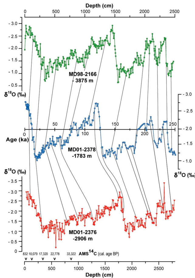
Figure 2. Planktonic oxygen isotopic record versus depth in core MD01-2376 and location of the five AMS 14 C dating (see Table 1). The studied core was correlated with the planktonic δ 18 O record of the neighbor core MD01-2378 [Holbourn et al., 2005]. The previously published age model of core MD98-2166 [Moreno et al., 2008] was revised using core MD01-2378 as reference. Solid lines join the tie points used for correlation.
