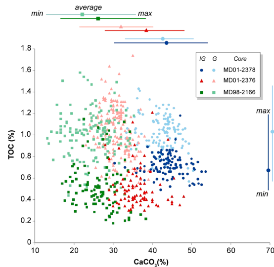
Figure 5. Organic carbon versus carbonate contents for the three selected cores (note that corrected \text{CaCO}_3 values are plotted for core MD01-2378) with respect to warm and cold periods. As expected, \text{CaCO}_3 content decreases with water depth due to carbonate dissolution. During interglacial (IG) periods, TOC content shows also a slight decrease with water depth as a consequence of the degradation of organic matter in oxic waters. During glacial (G) periods, TOC content increases and is even constant, whatever the water depth, as a result of increasing primary production and its exportation through the water column and a better preservation of organic compounds under dysoxic waters.
