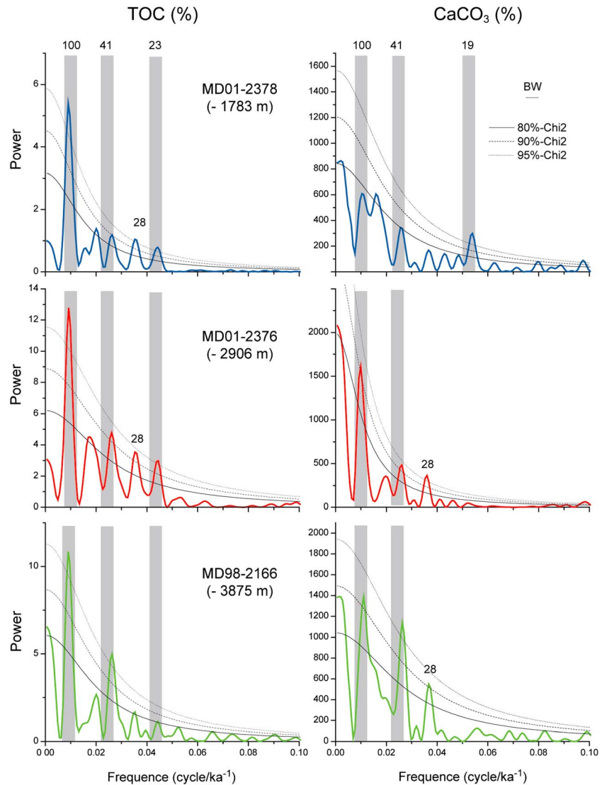
Figure 6. RedFit spectral analysis for the TOC and CaCO 3 records on the three selected cores for the last 240 ka.
