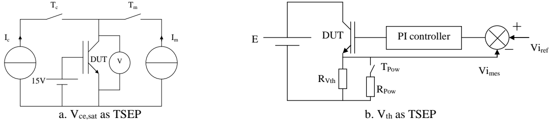
Fig. 4. Different methods for carrying out chip temperature measurements
