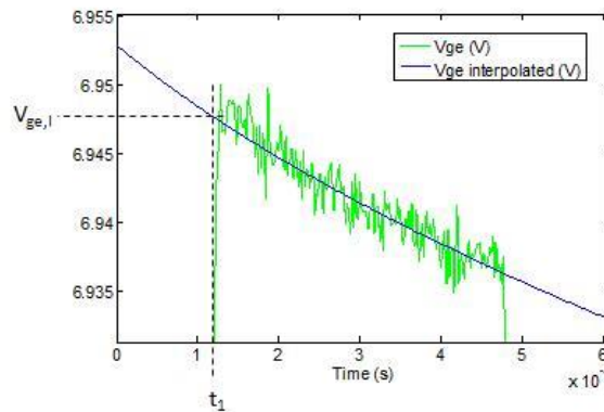
Fig. 10. Self-heating and interpolation of V_{ge} (cold plate temperature 40°C and E=20V )
