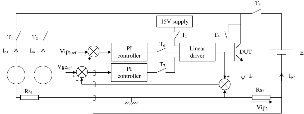
Fig. 5. Description of the electronic circuit
