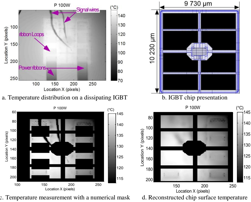
Fig. 6. Principle of the IR measurements
