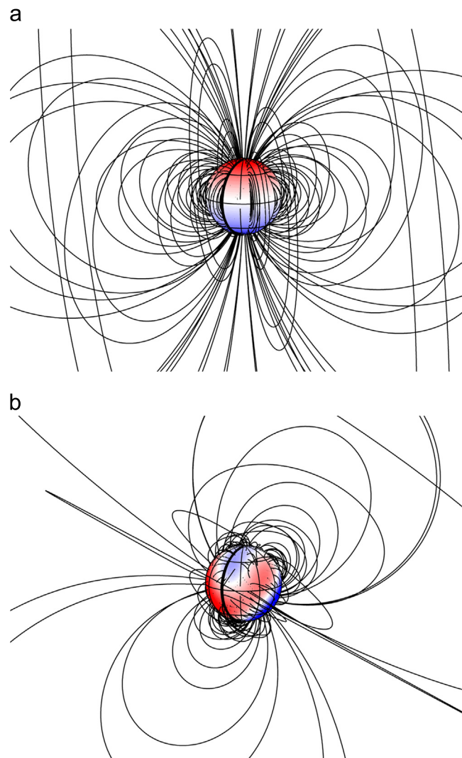
Fig. 3. Comparison of Uranus' highly asymmetrical field with Saturn's symmetrical field using the models of Herbert (2009) and Davis and Smith (1990), respectively. The colour scale indicates the magnitude of the radial field at the 1 bar level. (a) Saturn field (Davis and Smith, 1990) and (b) Uranus field (Herbert, 2009).
