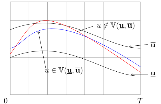
Fig. 1. An illustration of the set \mathbb{V}(\underline{u}, \bar{u}) in the case where l = 1
