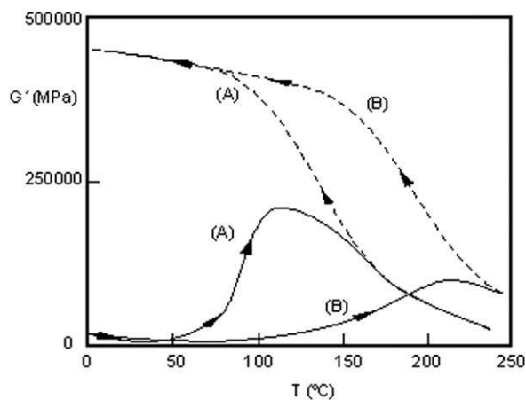
Figure 9. Modulus versus temperature curves for starting samples (full lines) and homogenized samples (dashed lines) for a light plasticizer (A) and a heavy plasticizer (B).
