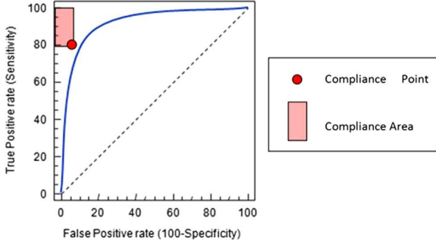
Fig. 4. Compliance point and compliance area on a ROC curve.
