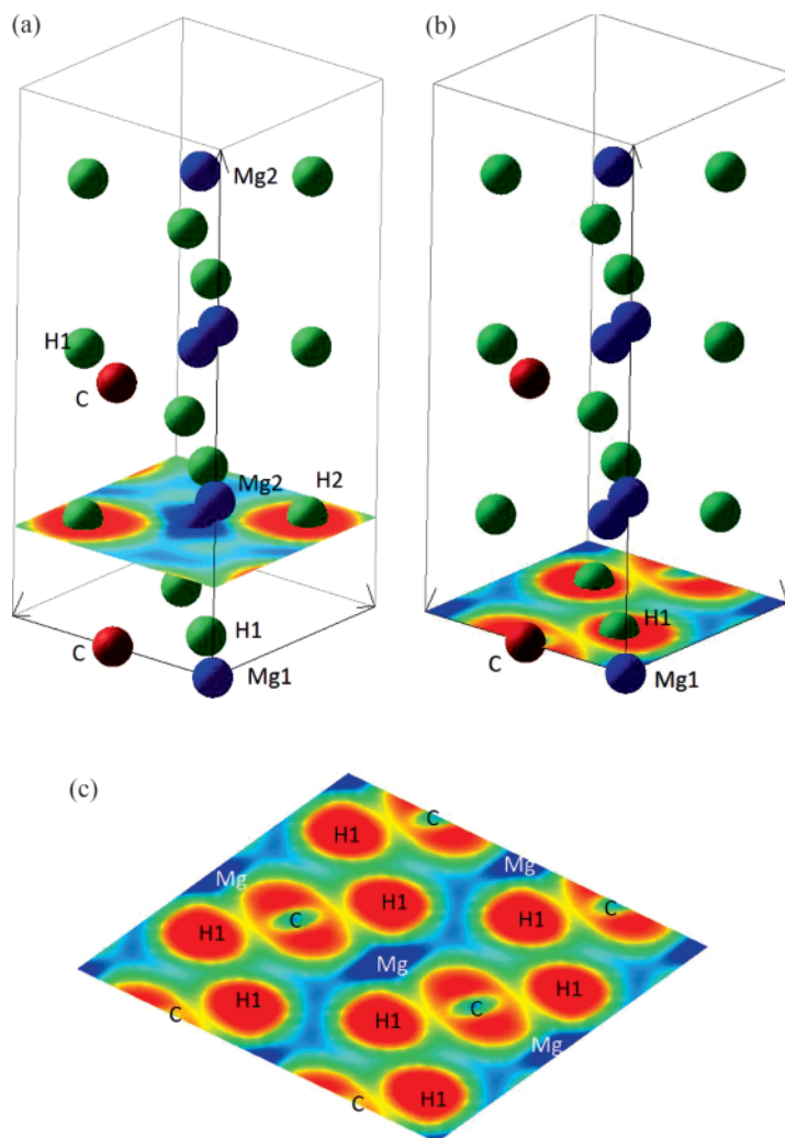
Fig. 5 (color online). Trirutile model structure for MgH 2 with electron localization function (ELF) slices perpendicular to the crystallographic c axis showing planes at a) Mg 2 , H 2 and b) at Mg 1 , H 1 with carbon; c) extended ELF slice over 4 cells comprising Mg 2 , H 1 and C.
