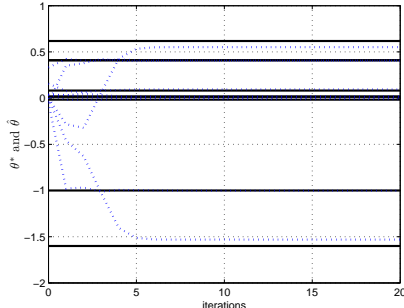
Fig. 3. Improvement after each iteration with procedure 3
