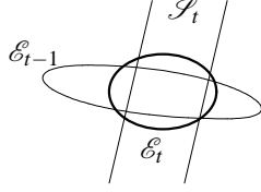
Fig. 1. 2-Dimensional example: (\mathcal{S}_t \cap \mathcal{E}_{t-1}) \subset \mathcal{E}_t
