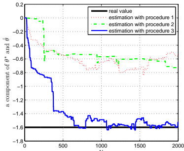
Fig. 2. Simulation results on the sixth component of \theta^*
