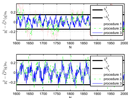
Fig. 4. Output errors and threshold \Delta_{v_t}
