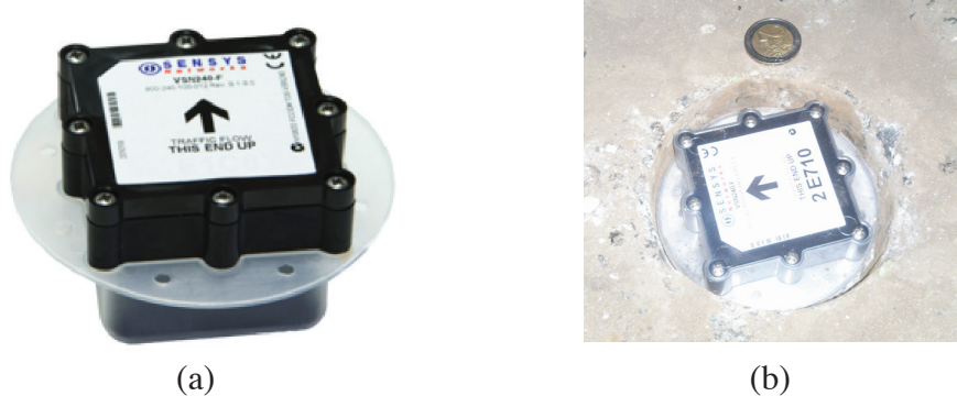
Figure 4. Magnetic sensors. (a) Sensys Networks VDS240 protected by a hardened plastic case (With permission of Sensys Networks, Inc.); (b) A magnetometer in its final location in the south ring, about 3 cm below the road surface, before being covered with fast-drying epoxy (the arrow points in the direction of traffic flow). A 2 Euro coin is shown near the sensor for comparison: the actual size is 7.4 cm \times 7.4 cm \times 4.9 cm and the weight is 300 grams.
