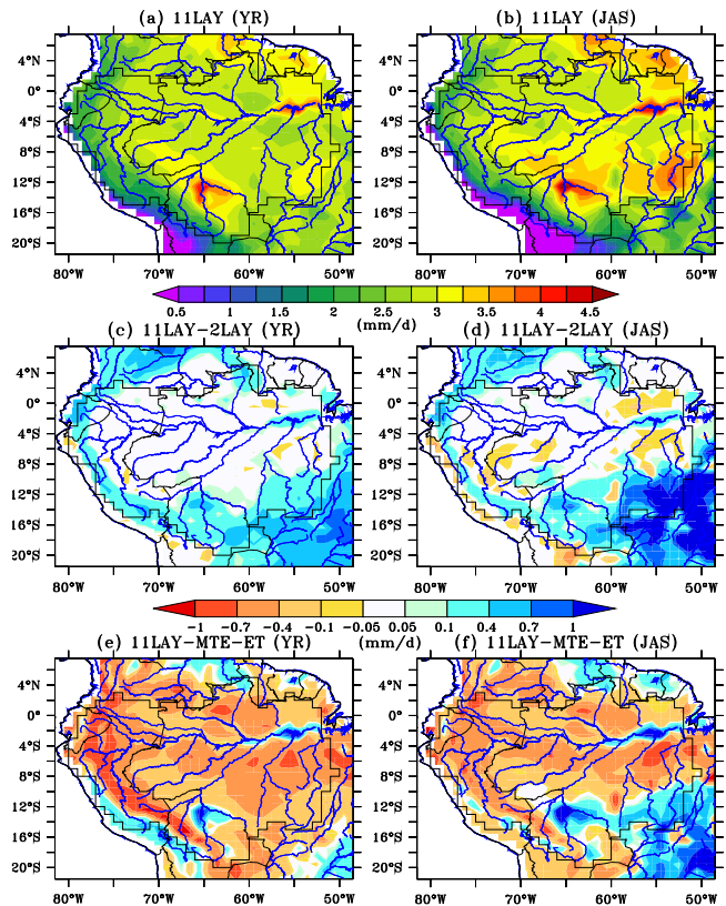
Figure 5. Mean ET ( \text{mm d}^{-1} ) simulated by the 11LAY, averaged over (a) the complete year and (b) JAS, averaged over the period 1980–2008. Differences in simulated ET between the 11LAY and (c, d) the 2LAY and (e, f) the MTE-ET product.
