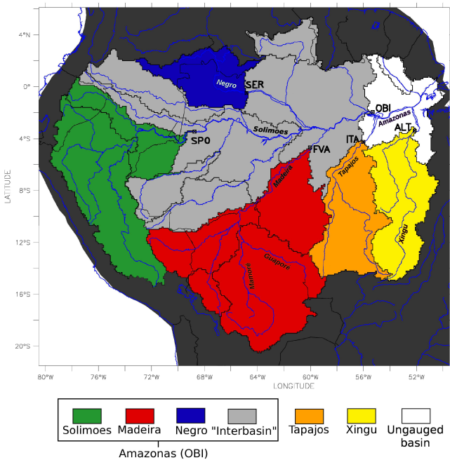
Figure 1. Map of the Amazon sub-basins and their gauging stations. Color is used to indicate the sub-basins studied here. Modified from Guimberteau et al. (2012a).
