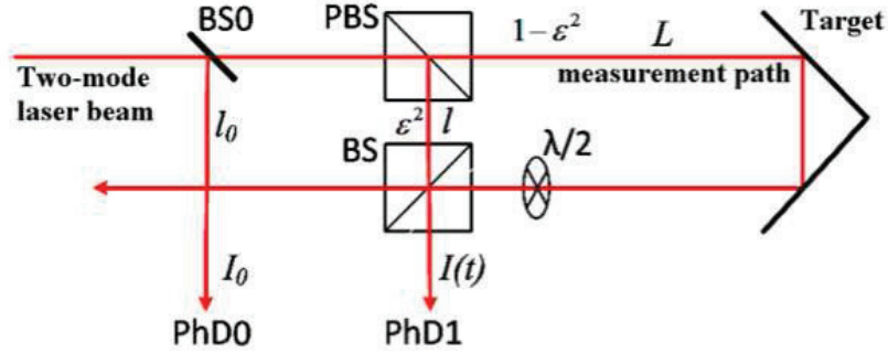
Figure 1.: Schematic diagram of the telemeter. BSO: beam splitter plate; (P)BS: (polarizing) beam splitter cube.
