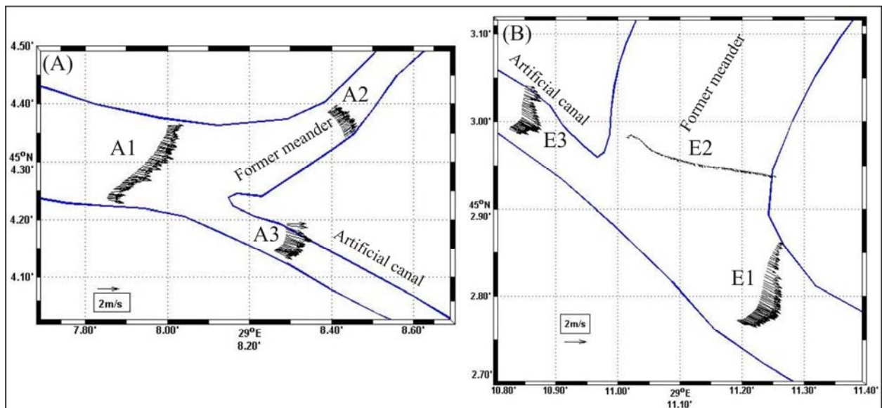
Fig. 6. aDcp depth-averaged velocities and river-bank contours within sectors of (A) bifurcation and (B) confluence. Channel contours were digitized from a satellite image dating from June 2000 for different hydrological conditions than during the measurement period
