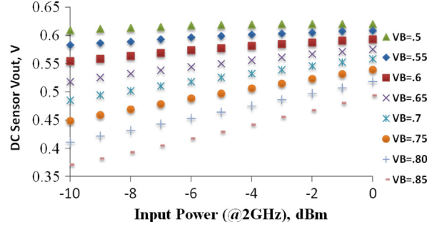
Fig. 15. Evolution of the embedded temperature sensor output voltage as a function of the PA input power for different V_B ( V_{DD}=1.2 \text{ V} ).
