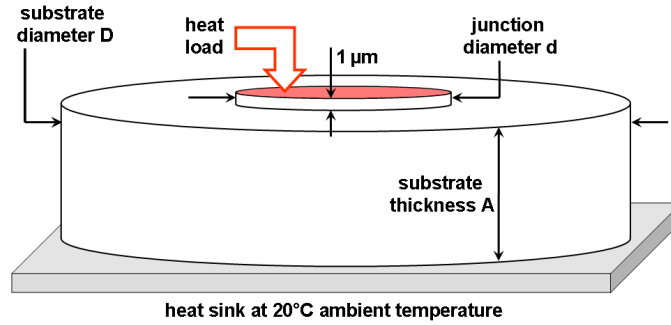
Fig. 9: Geometry of the junction/substrate/heat sink assembly used for the simulations. Drawing is not to scale. The heat load is applied uniformly on the top side of the 1 \mu\text{m} thick cylinder that simulates the photodetector junction.
