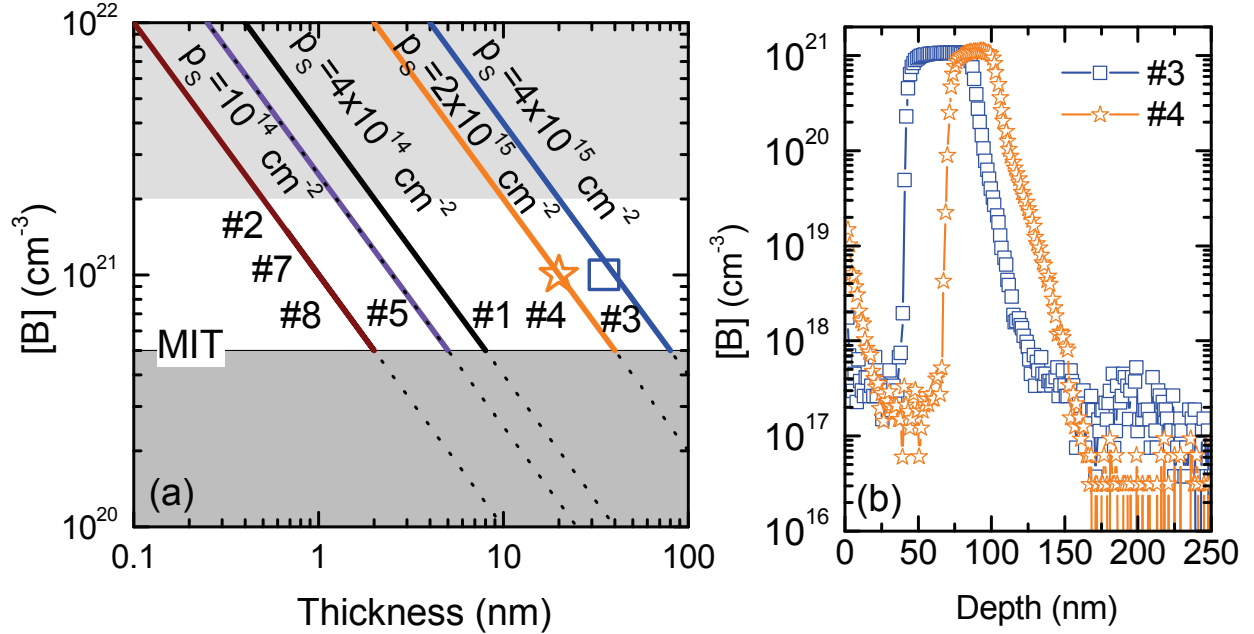
FIG. 12. (a) Sheet carrier density isolines measured by Hall effect, drawn on a boron concentration (cm -3 ) versus thickness (nm) plot. For [B] \geq 5 \times 10^{20} cm -3 the conduction is metallic. An upper limit was drawn at 2 \times 10^{21} cm -3 (see text). The intercepts of the lines (boundaries between full and dashed) with the horizontal line corresponding to the critical concentration for the MIT yield the maximum thickness of the highly doped region where [B] > 5 \times 10^{20} cm -3 , while the intercept of the lines with [B] = 2 \times 10^{21} cm -3 gives the minimum possible thickness. The symbols are SIMS data for samples #3 (square) and sample #4 (star). (b) SIMS boron depth profiles (Cs + at 15 keV) of the two thickest p^{++} layers discussed in this work (#3 and #4).
