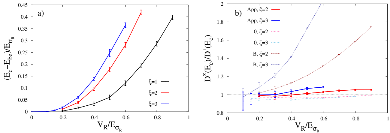
Figure 2. (Color online) (a) Position of the mobility edge with respect to the band edge E_c - E_{be} as a function of the amplitude of the disorder in the approximation (6), for geometrical anisotropies \xi = 1, 2 and 3 (black, red and blue data points respectively). (b) Anisotropy of the diffusion tensor at the mobility edge found within the approximation for \xi = 2 and 3 (red and blue data resp.), compared with the anisotropy of \mathbf{D}_0 and \mathbf{D}_B at the same energy (light dashed and dark dotted lines resp.).
