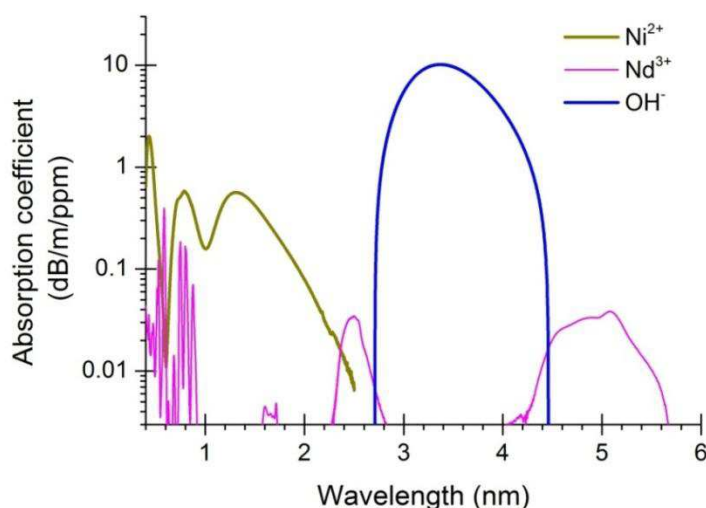
Figure 1. Comparison of absorption coefficients of some selected impurities in a conventional tellurite glass (composition: 75\text{TeO}_2\text{--}20\text{ZnO}\text{--}5\text{Na}_2\text{O} , mol.%) (summarized from results in Reference [13].)
