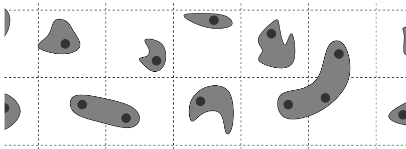
Figure 1.d): An example where (NCC) holds but (GCC) does not. A network of balls where the damping is effective is in dark grey. In this case, the exponential decay of Theorem 1.2 fails but the logarithmic decay of Theorem 1.3 holds.
