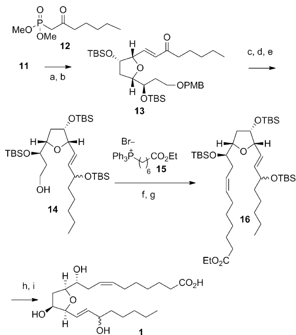
Scheme 5. Reagents and conditions: a) DMP, \text{CH}_2\text{Cl}_2 , RT; b) Ba(OH) 2 , THF, RT, 60% over two steps; c) \text{CeCl}_3 \cdot 7\text{H}_2\text{O} , NaBH 4 , MeOH, 0°C; d) TBSCl, imidazole, DMAP, \text{CH}_2\text{Cl}_2 , RT, 85% over two steps; e) DDQ, \text{CH}_2\text{Cl}_2/\text{H}_2\text{O} (10:1), 0°C to RT, 80%; f) DMP, \text{CH}_2\text{Cl}_2 , RT; g) 15 , NaHMDS, THF, -78°C to RT, 65% over two steps; h) TBAF, THF, RT; i) LiOH, THF/ \text{H}_2\text{O} (1:1), RT, 76% over two steps. DMP = Dess–Martin periodinane, DDQ = 2,3-dichloro-5,6-dicyano-1,4-benzoquinone, NaHMDS = sodium bis(trimethylsilyl)amide, TBAF = tetrabutylammonium fluoride.
