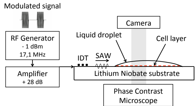
Fig. 1 Schematic diagram of the setup showing the cell layer (red dashed line) immersed in a 20 μl PBS droplet atop a LiNbO 3 piezoelectric substrate. The diagram also shows the interdigitated transducers (IDT), RF amplifier and signal generator used for Rayleigh type SAW generation. Cell visualization is achieved using a phase contrast phase microscope, 10× objective, and CMOS camera.
