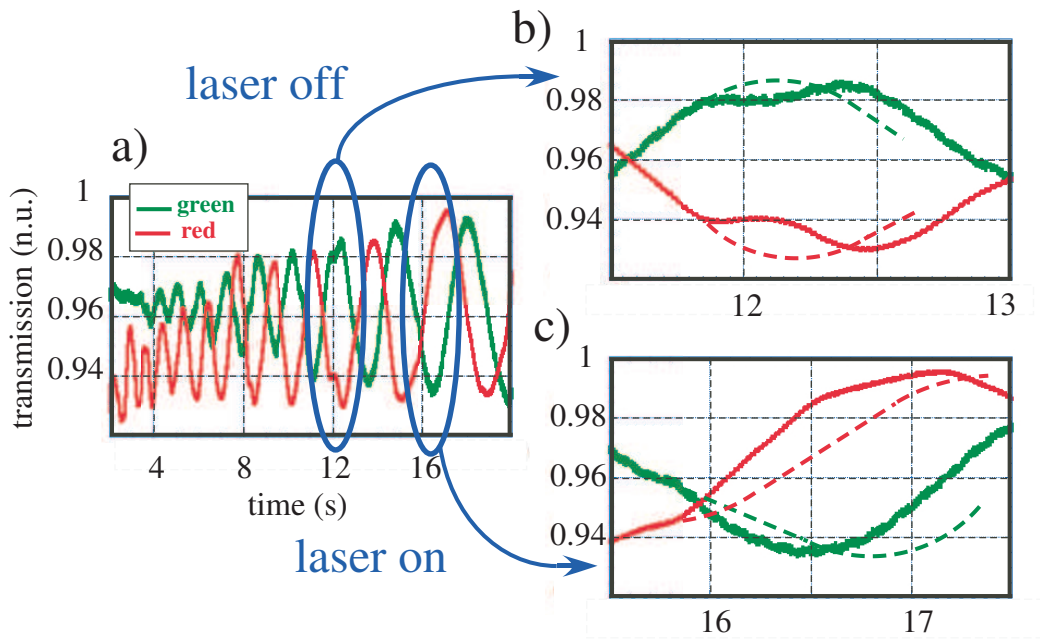
FIG. 2. Deformation of the film interfaces. Interference transmission fringes during the drainage of the film, while the modulated laser is switched on and off several times (a). n.u.: normalized unities. Zoom on the fringes for two specific cases (b), laser off and (c), laser on). The dotted lines are a prolongation of the evolution of the fringes without the applied perturbation. We estimate that the interface deformation is of the order of 20 nm when the laser is either on or off.
