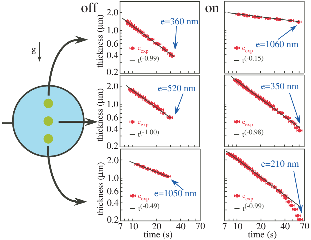
FIG. 4. Drainage curves of the film without and with the laser modulation, at resonance. Thickness evolution of the film versus time at the top, middle and bottom of the frame, without and with the laser modulation, on a log-log scale. The laser modulation frequency equals 23.5 Hz. The red points are experimental values together with the error bars due to the statistic, each measurement being performed three times. The black solid line is a power fit. The absolute precision on the power law is 0.03.
