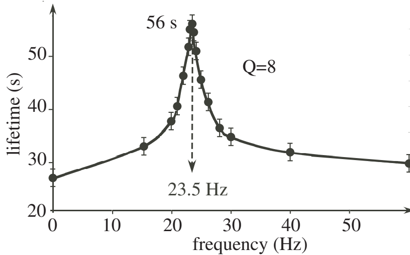
FIG. 3. Lifetime of the film versus modulation frequency. A resonance behaviour of the lifetime of the film for around a 23.5 Hz frequency modulation of the laser beam is evidenced. The quality factor Q equals 8. The lifetime of the film is more than doubled at resonance.
