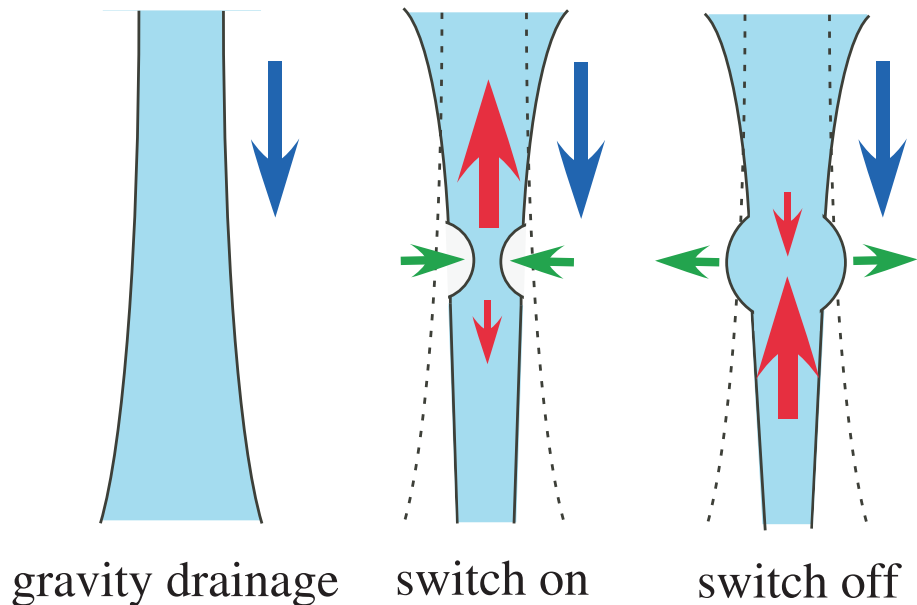
FIG. 5. Influence of the laser on the interfaces (green arrow), flow of the liquid in the film (red arrow) and influence of gravity (blue arrow). The deformations are exaggerated. Left drawing and dotted line: free standing draining film. Other drawings: laser on-laser off cycle. In the upper part of the film, the effect of gravity is hidden by the effect of the laser, leading to an inflation in the upper zone.
