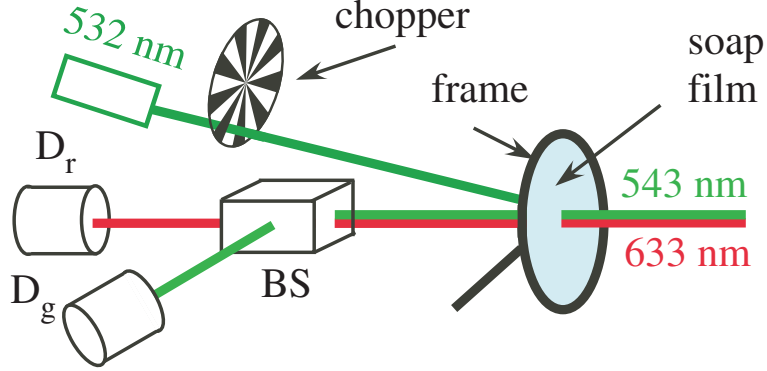
FIG. 1. Experimental set up. Laser light from a 532 nm -2 mW solid state laser deforms a vertical free standing thin soap film. The film thickness is measured from the transmission interferences of two low power lasers with different colors ( \lambda = 633 nm and \lambda = 543 nm). BS: beam splitter, D g and D r : photodiodes detecting green and red light respectively.
