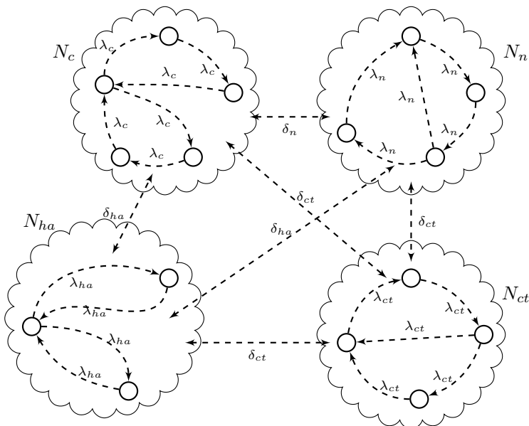
Figure 1: A schematic sketch of \mathcal{D}(A) of Example 3.4 (the general case)
