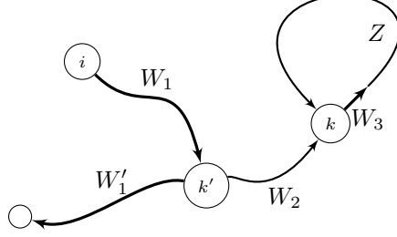
Figure 3: Walks \tilde{V} = W_1 W_1' and W = W_1 W_2 Z^r W_3 in proof of Theorem 4.6.
