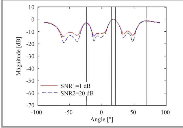
Fig. 2. Bartlett spectrum.
