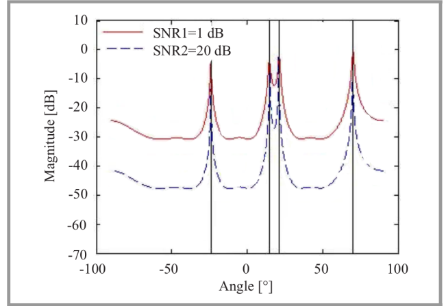
Fig. 8. MUSIC spectrum.
