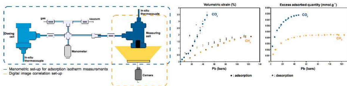
Fig. 2. Simultaneous in-situ measurements of swelling and adsorption on activated carbon filled with pure CO 2 and pure CH 4 at T = 30^\circ C .
