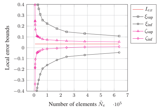
FIGURE 2. COMPARISON BETWEEN CLASSICAL AND NEW BOUNDINGS.
