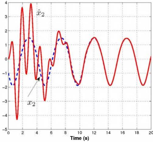
Fig. 4. Evolution of the second state for \tau = 0.5s with a cascade of 2 observers
