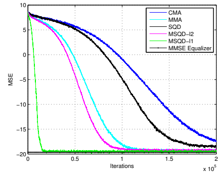
(a) 16-QAM
