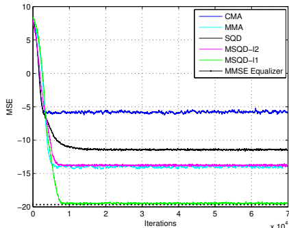
(a) 16-QAM
