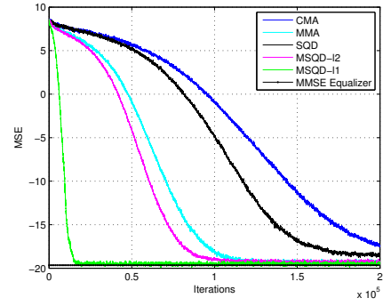
(a) 16-QAM
